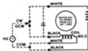
CONNECTION DIAGRAM LM0 Synchronous Motor
