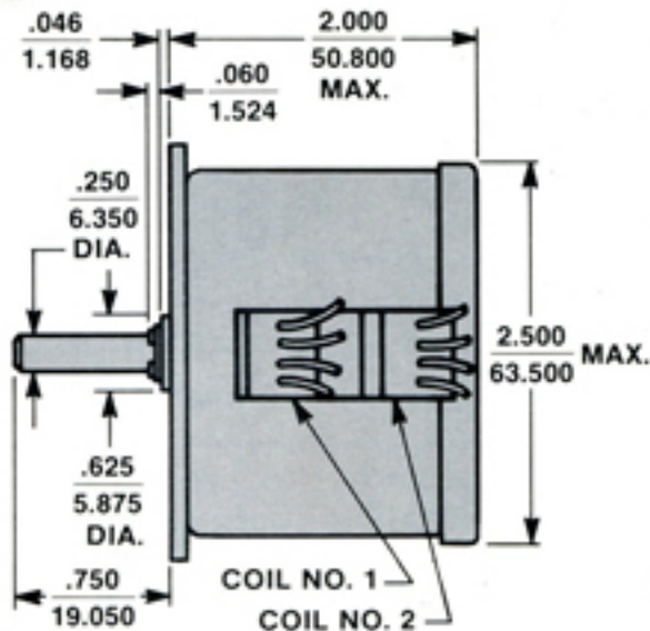
CONNECTION DIAGRAM LMS 7000 Stepper Motor
