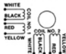
CONNECTION DIAGRAM LM0 Synchronous Motor
